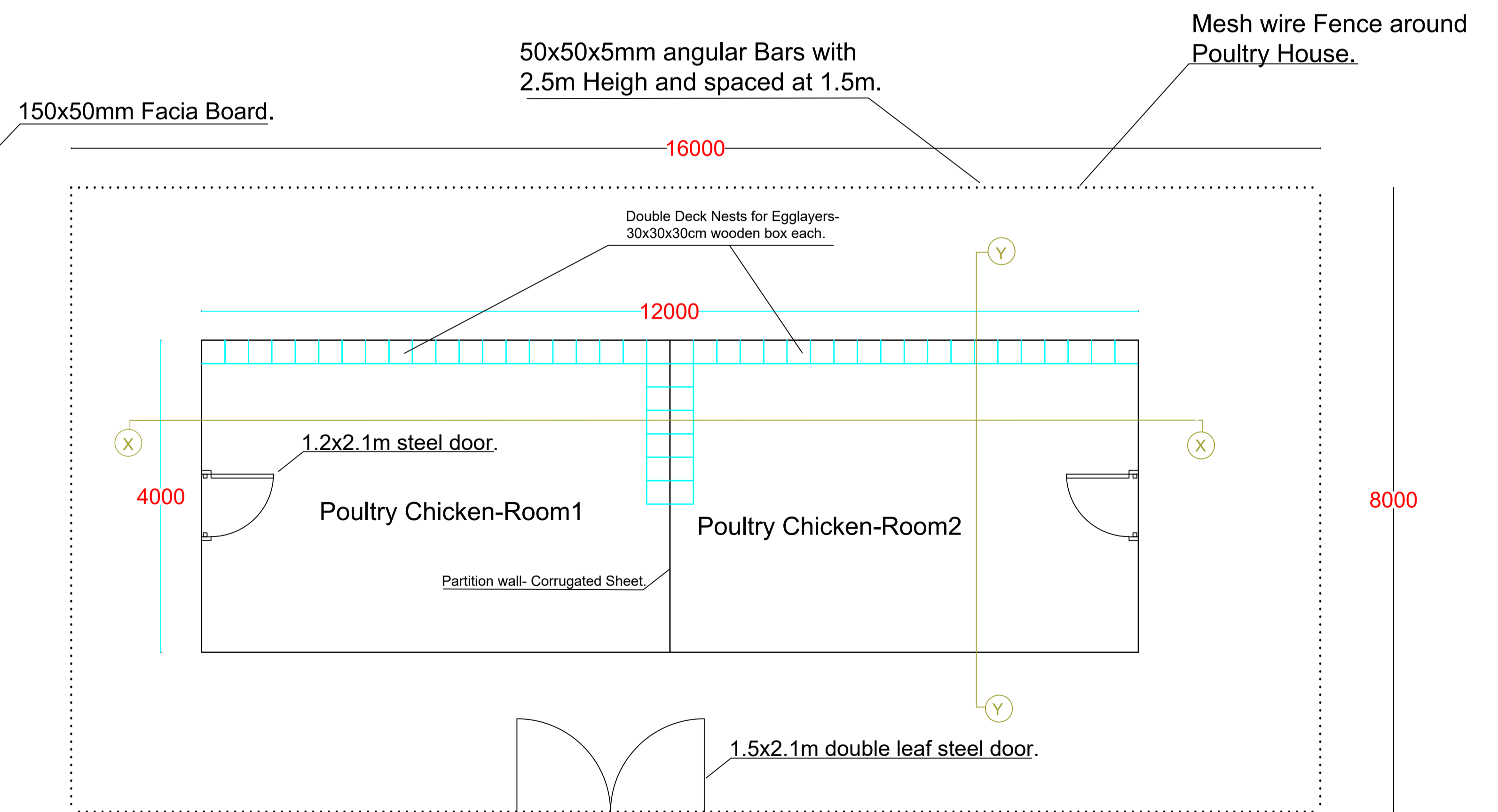
Poultry House Plan View.
