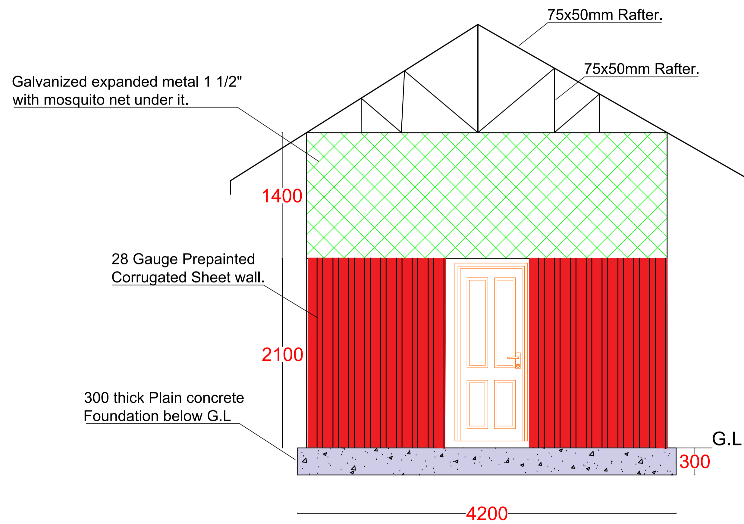
Poultry House-Section Y-Y.
