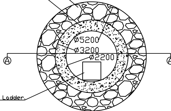
Cross section- Shallow well.
