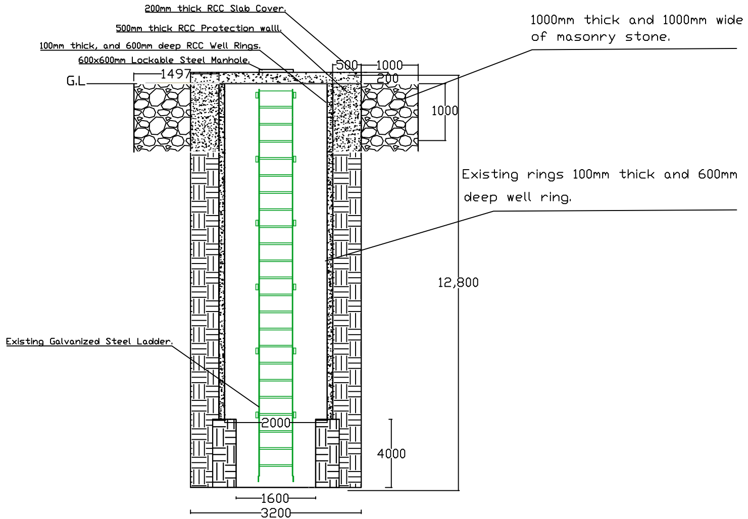
Vertical section A-A - Shallow well.
