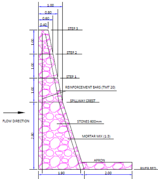
CROSS SECTION A-A SCALE 1:75
