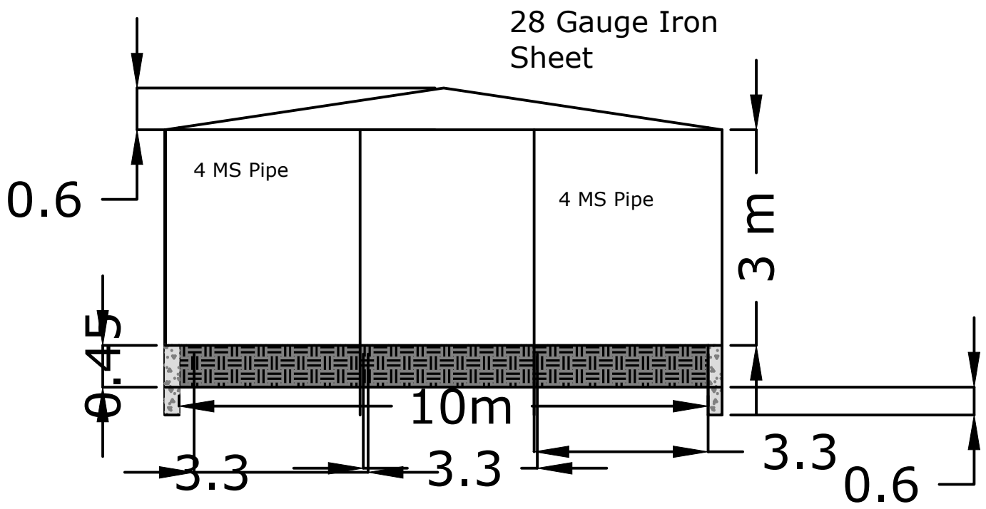
Section for Car parking for shade
