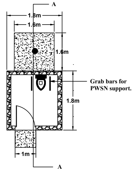
Floor plan.
