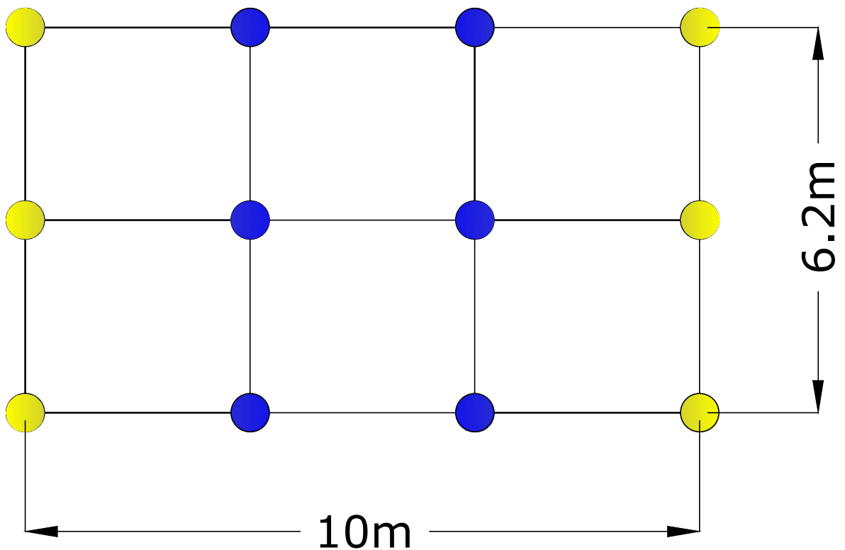
Design Layout plan for car parking shade
